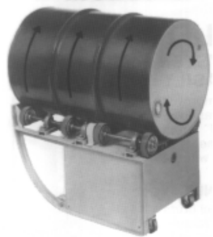
080H-001 Portable Drum Rotator
