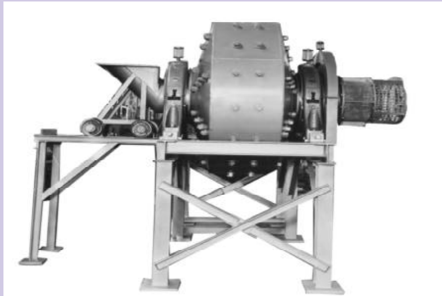
The 6' Diameter X 2' Long Continuous Feed Autogenous/Semi-Autogenous Mill With Base & Stand
